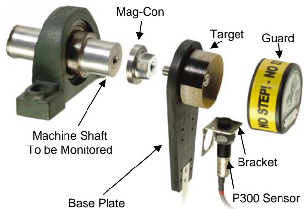
P300 Inductive Sensor shown with optional Whirligig and Mag-Con
